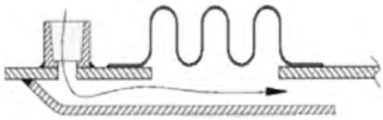
Purge Ports
