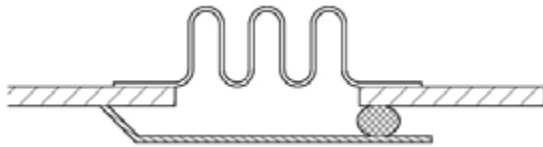
Packed Bellows
