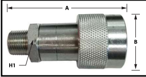
COUPLER - POPPET
