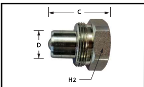
NIPPLE - BALL
