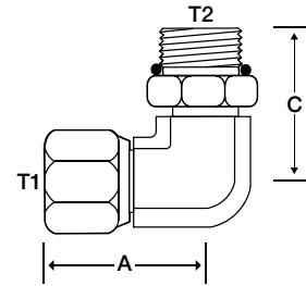
FS6809 FFX - MAORB 90°
